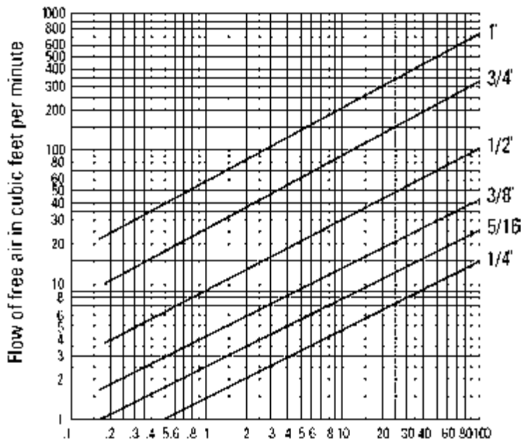
Pressure drop in pounds per sq. in., per 100 ft. of hose
